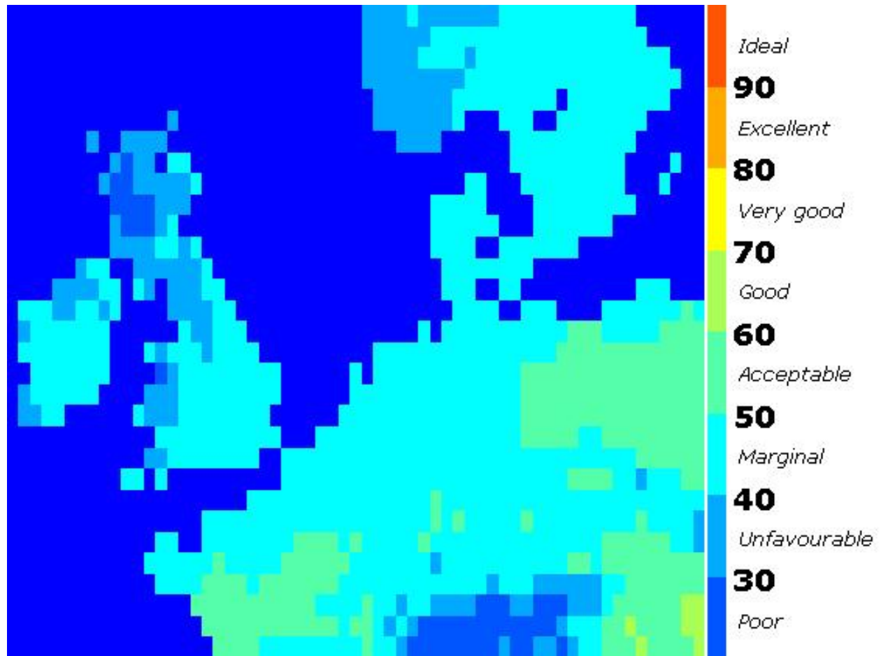
Figure 1. TCI Values for North-Western Europe (spring, 1970s)
