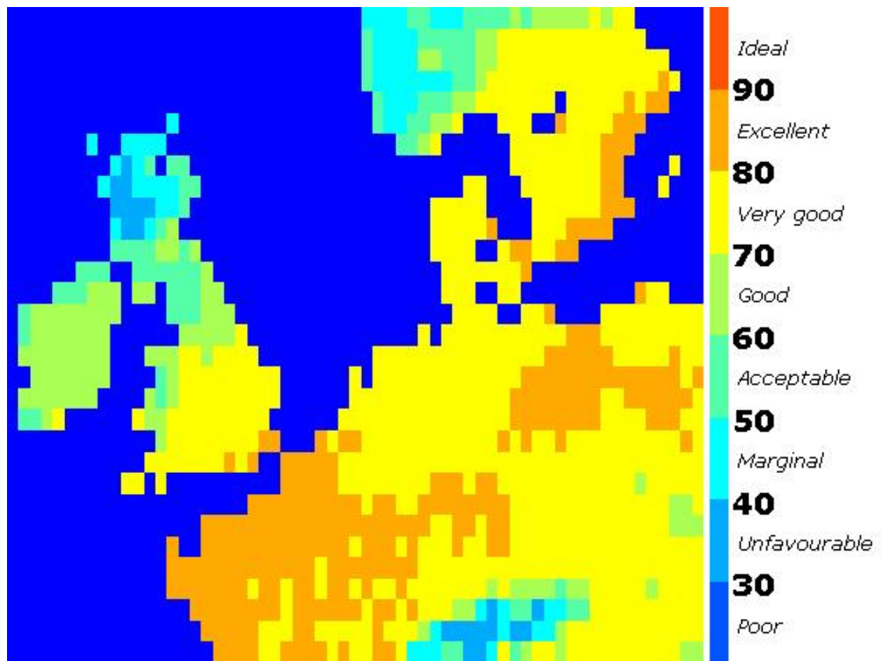
Figure 11. TCI Values for North-Western Europe (summer, 2050s, B1)
