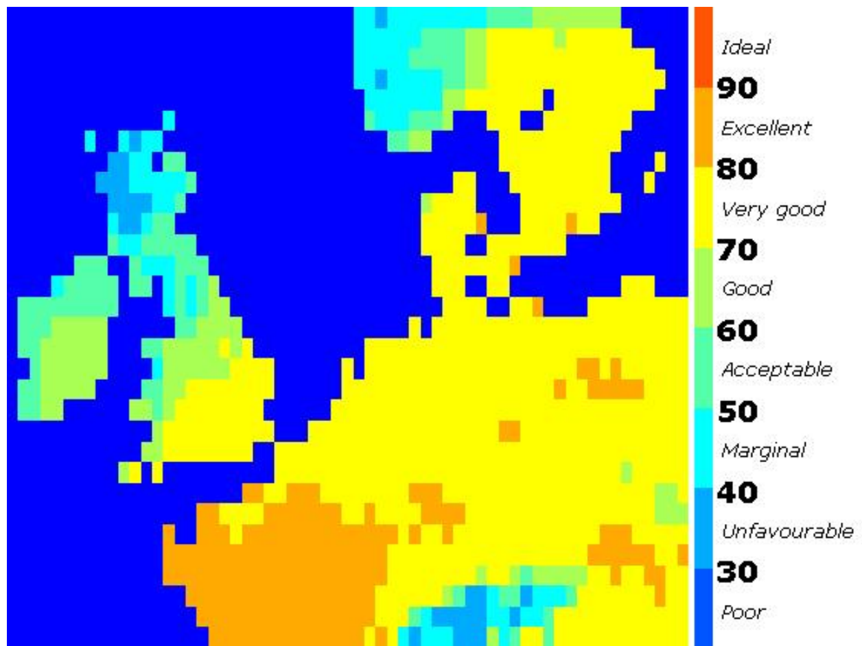
Figure 8. TCI Values for North-Western Europe (summer, 2020s, A1F)
