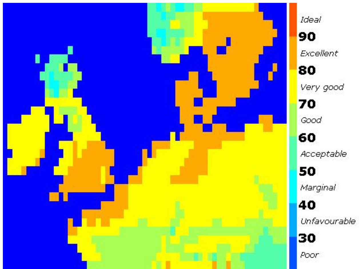
Figure 20. TCI Values for North-Western Europe (summer, 2080s, A1F)
