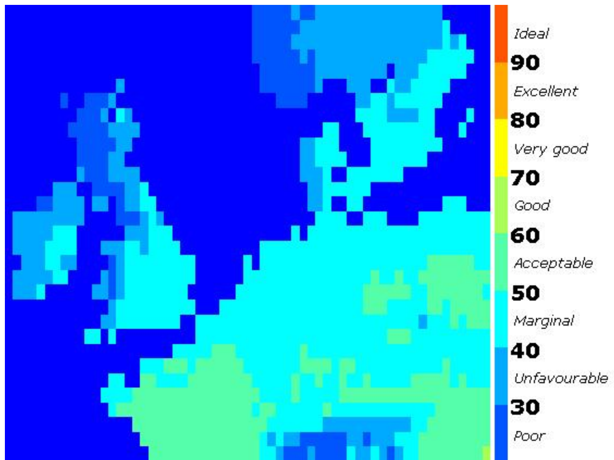
Figure 3. TCI Values for North-Western Europe (autumn, 1970s)
