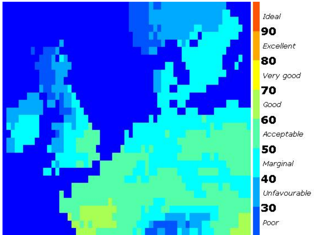
Figure 9. TCI Values for North-Western Europe (autumn, 2020s, A1F)
