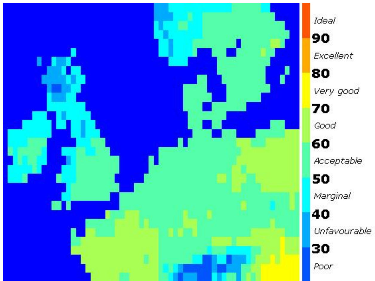
Figure 19. TCI Values for North-Western Europe (spring, 2080s, A1F)
