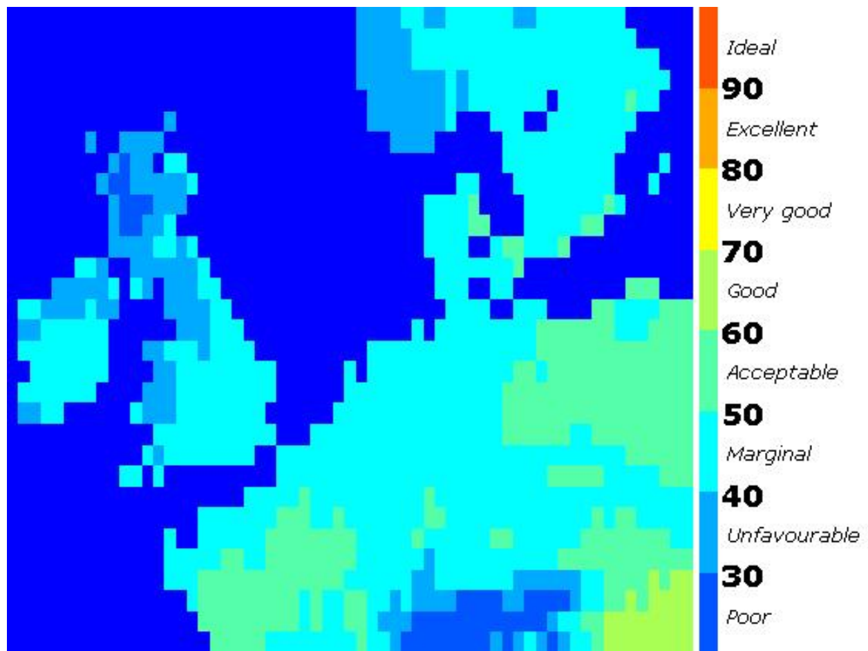
Figure 4. TCI Values for North-Western Europe (spring, 2020s, B1)
