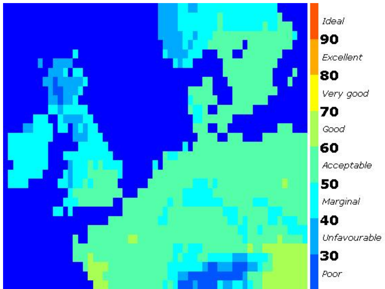
Figure 13. TCI Values for North-Western Europe (spring, 2050s, A1F)
