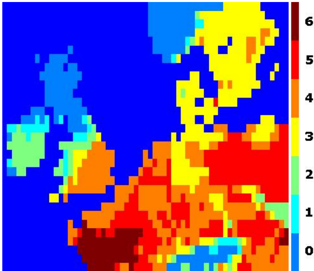
Figure 27. Number of Acceptable Months ( TCI \geq 70 ) in North-Western Europe (2080s, B1)
