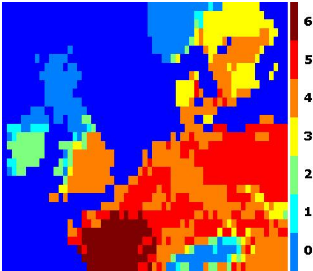
Figure 26. Number of Acceptable Months ( TCI \geq 70 ) in North-Western Europe (2050s, A1F)
