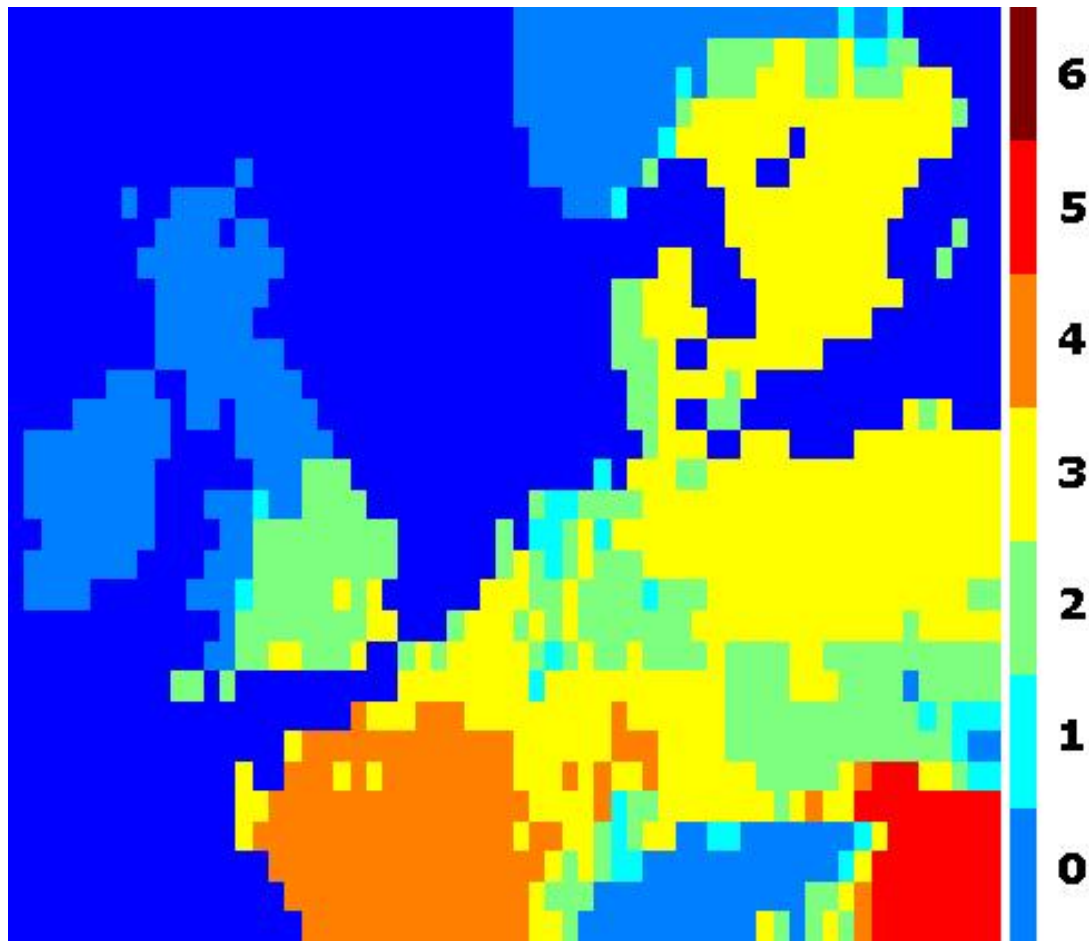
Figure 23. Number of Acceptable Months ( TCI \geq 70 ) in North-Western Europe (2020s, B1)
