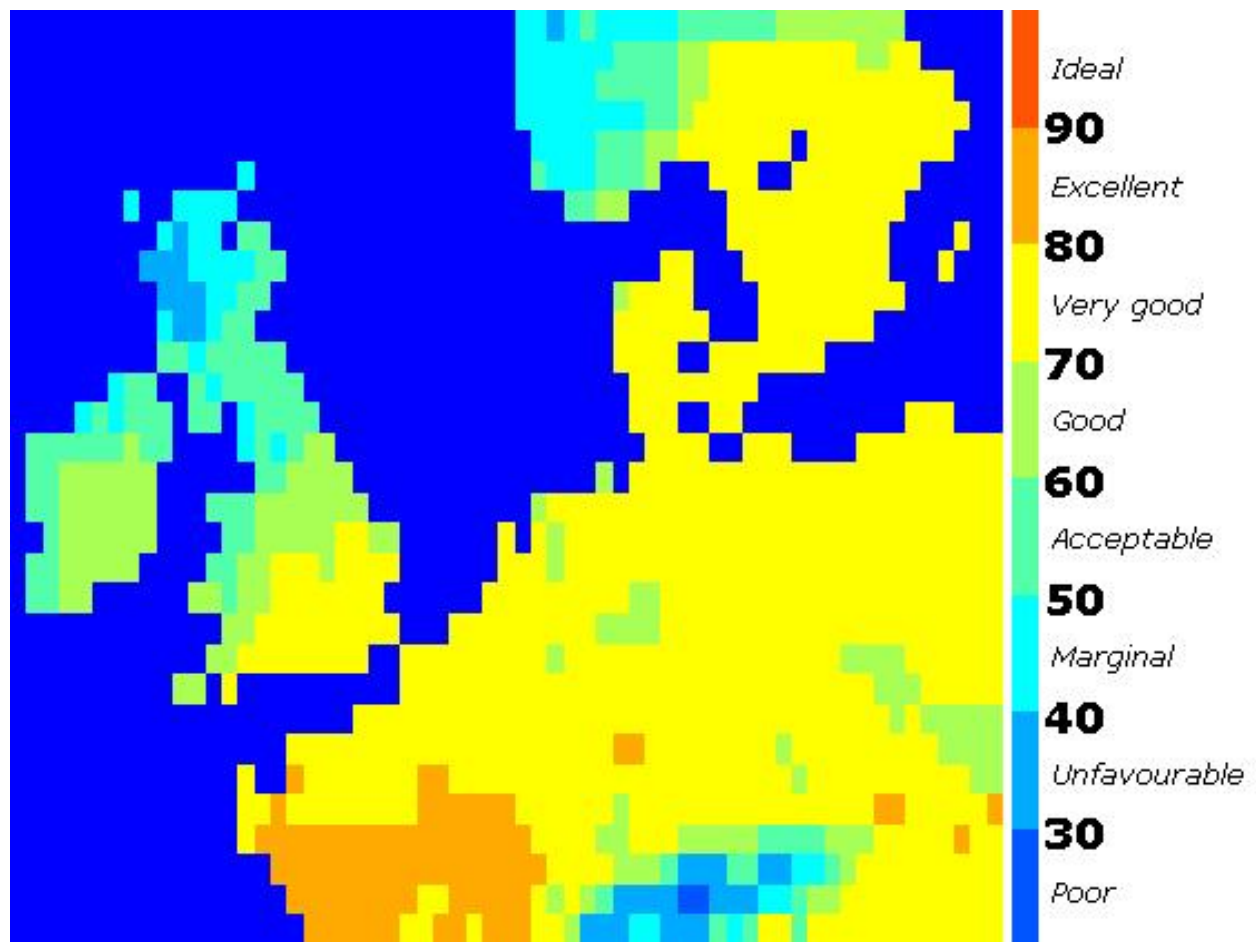
Figure 5. TCI Values for North-Western Europe (summer, 2020s, B1)
