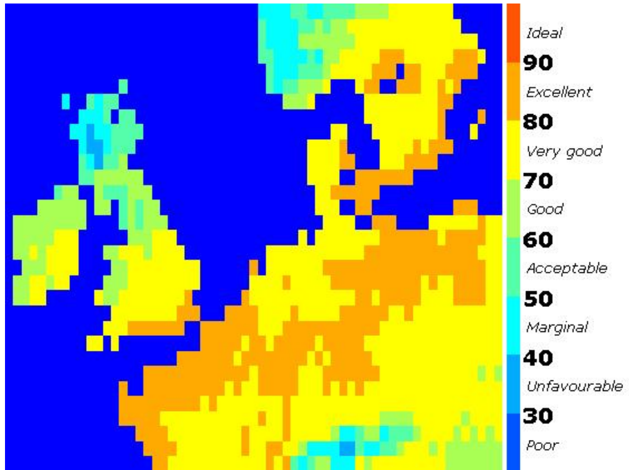
Figure 17. TCI Values for North-Western Europe (summer, 2080s, B1)
