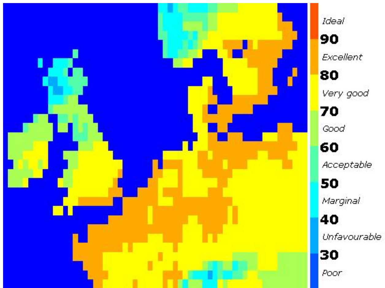
Figure 14. TCI Values for North-Western Europe (summer, 2050s, A1F)
