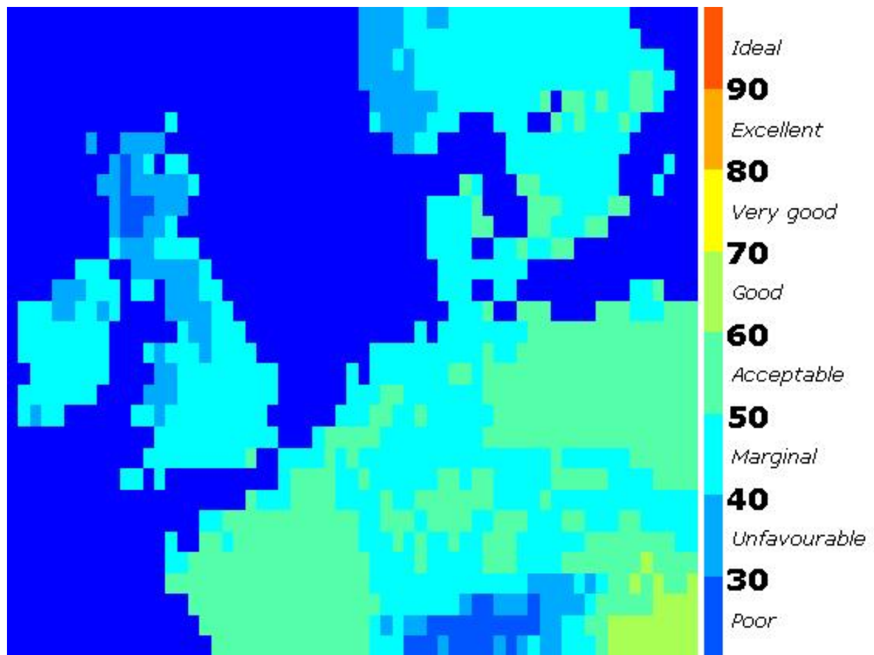
Figure 7. TCI Values for North-Western Europe (spring, 2020s, A1F)
