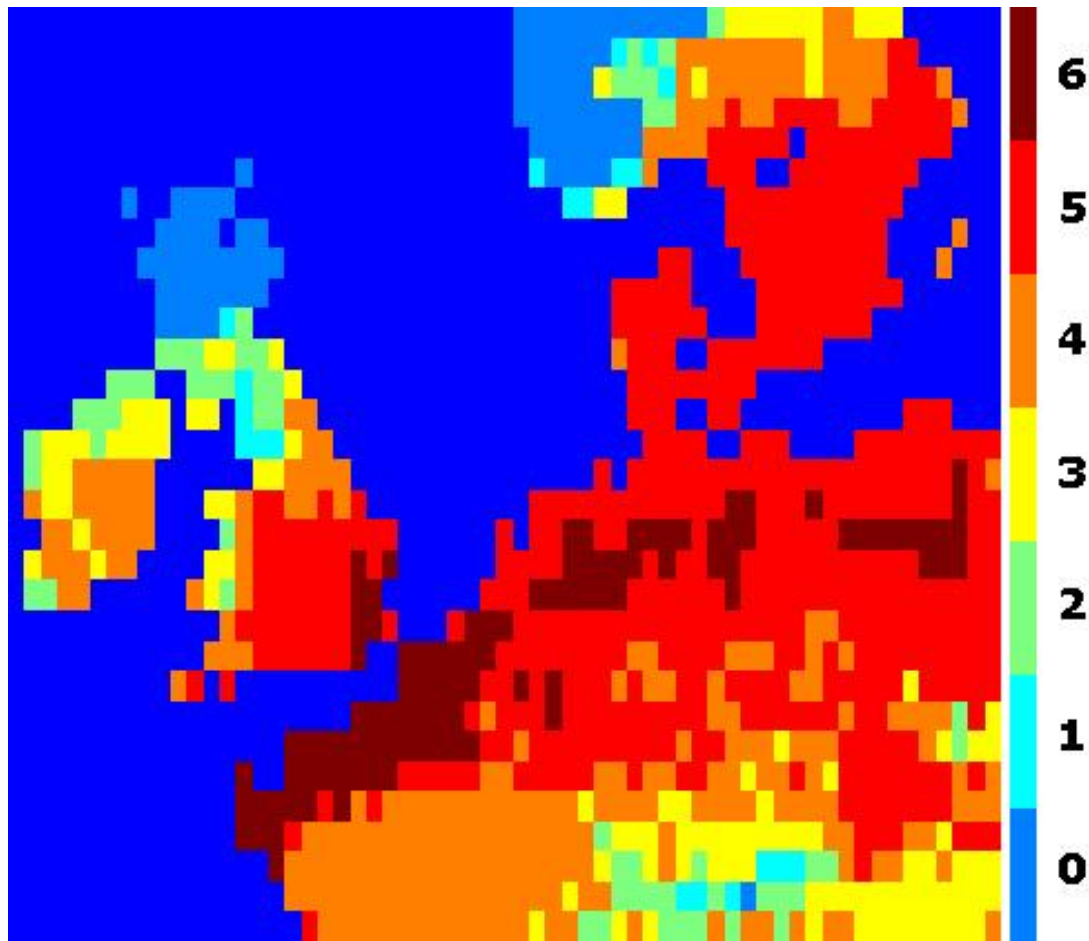
Figure 28. Number of Acceptable Months ( TCI \geq 70 ) in North-Western Europe (2080s, A1F)
