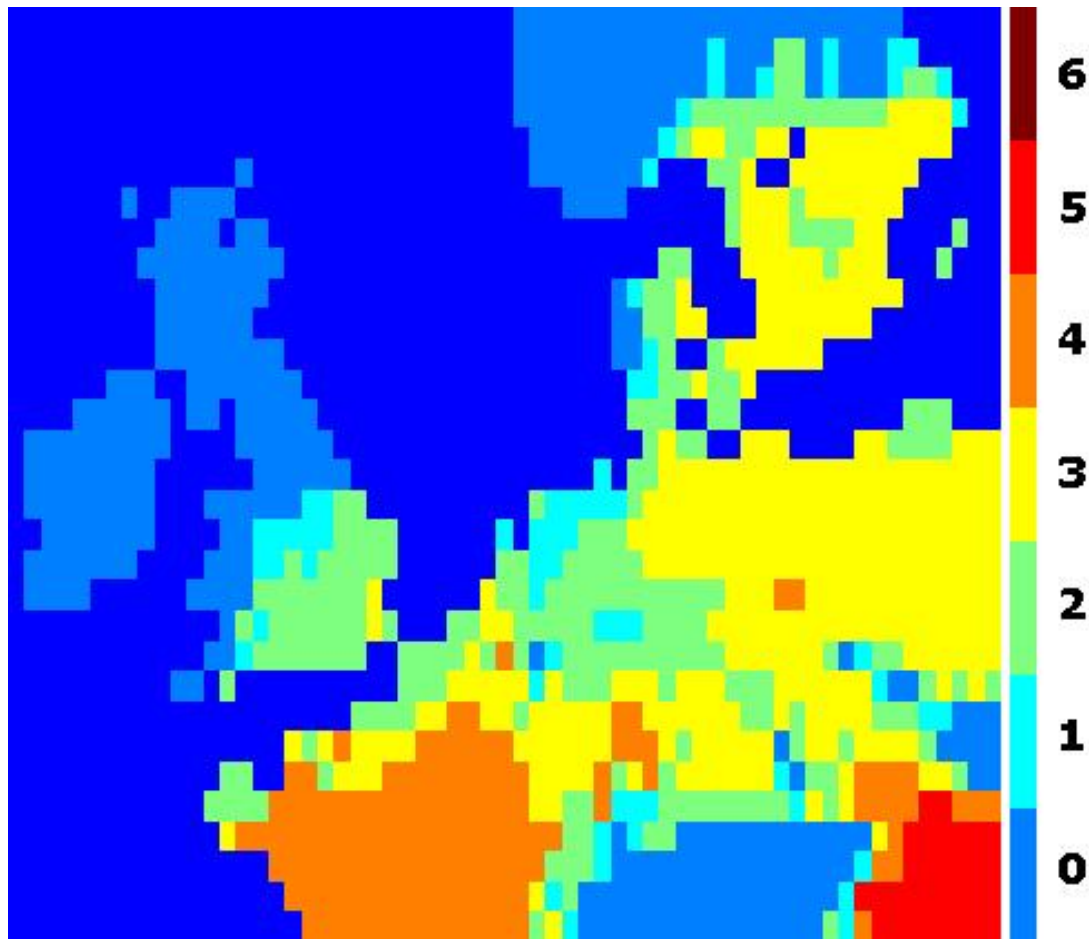
Figure 22. Number of Acceptable Months ( \text{TCI} \geq 70 ) in North-Western Europe (1970s)
