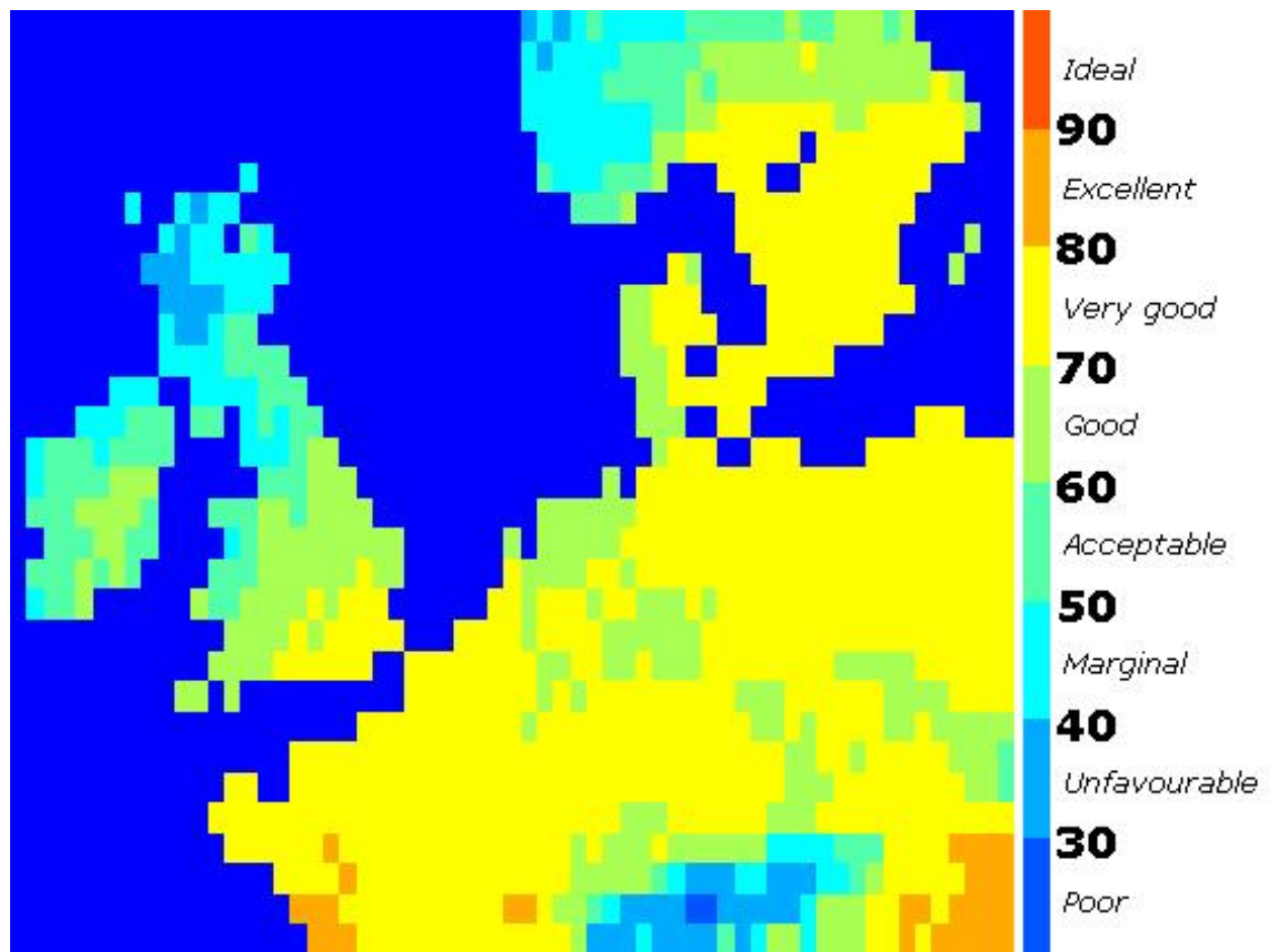
Figure 2. TCI Values for North-Western Europe (summer, 1970s)
