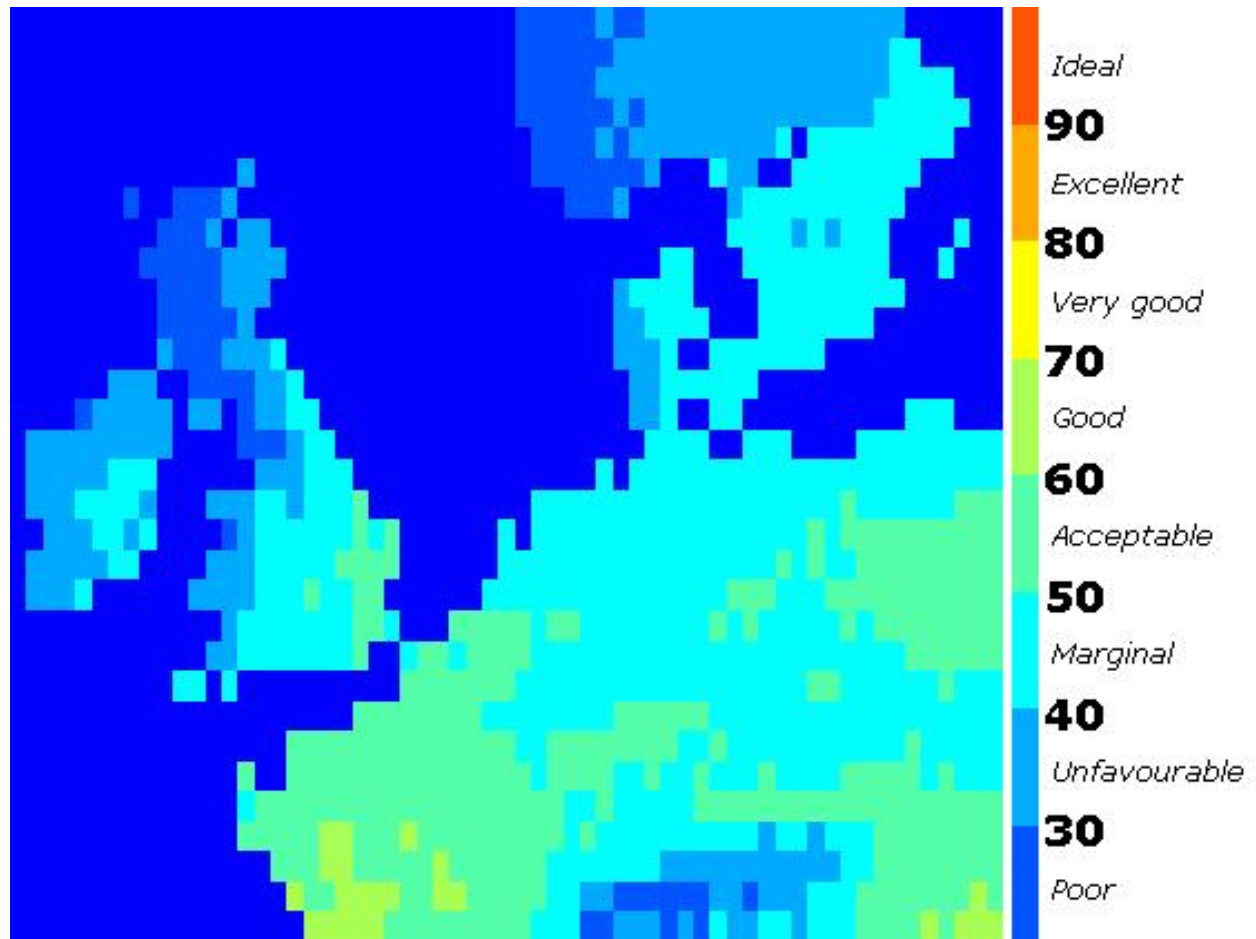
Figure 6. TCI Values for North-Western Europe (autumn, 2020s, B1)
