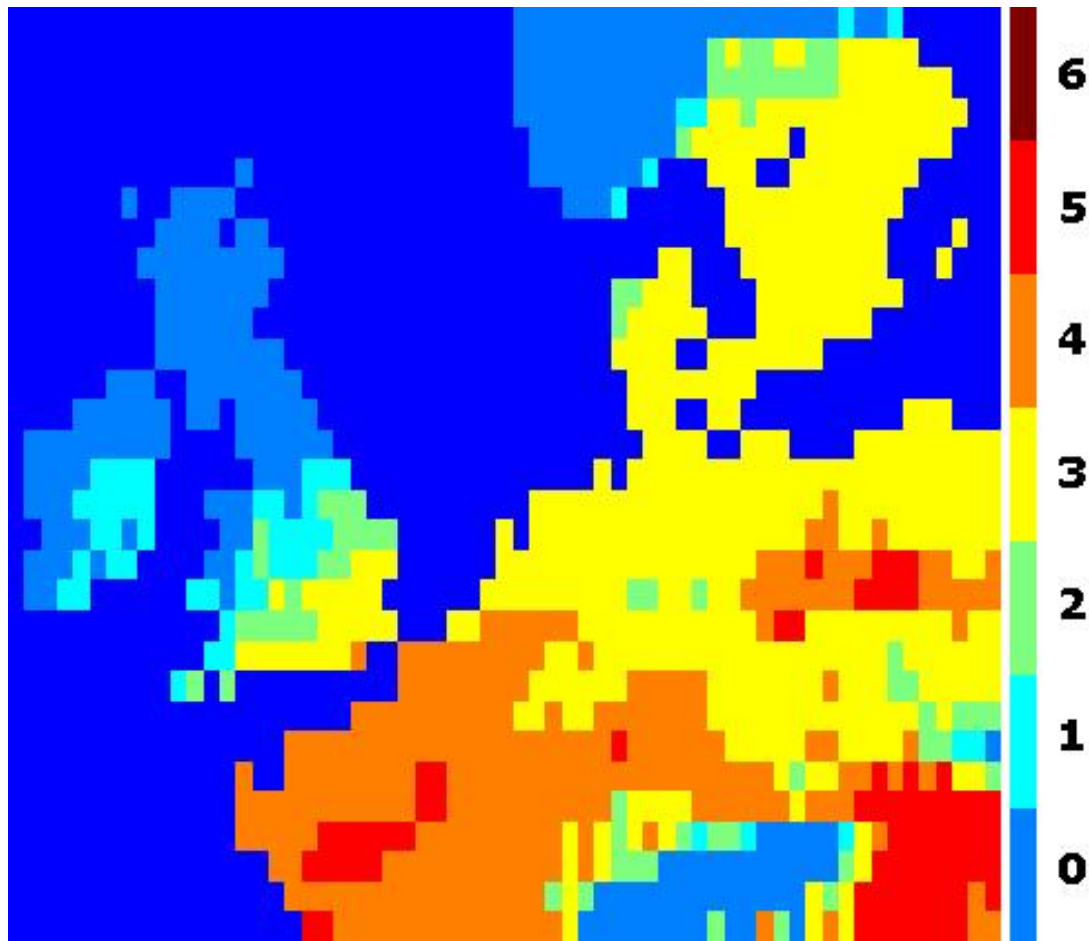
Figure 24. Number of Acceptable Months ( TCI \geq 70 ) in North-Western Europe (2020s, A1F)
