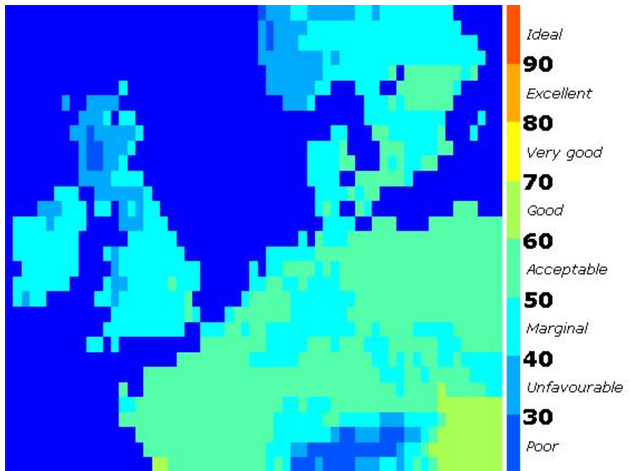
Figure 10. TCI Values for North-Western Europe (spring, 2050s, B1)
