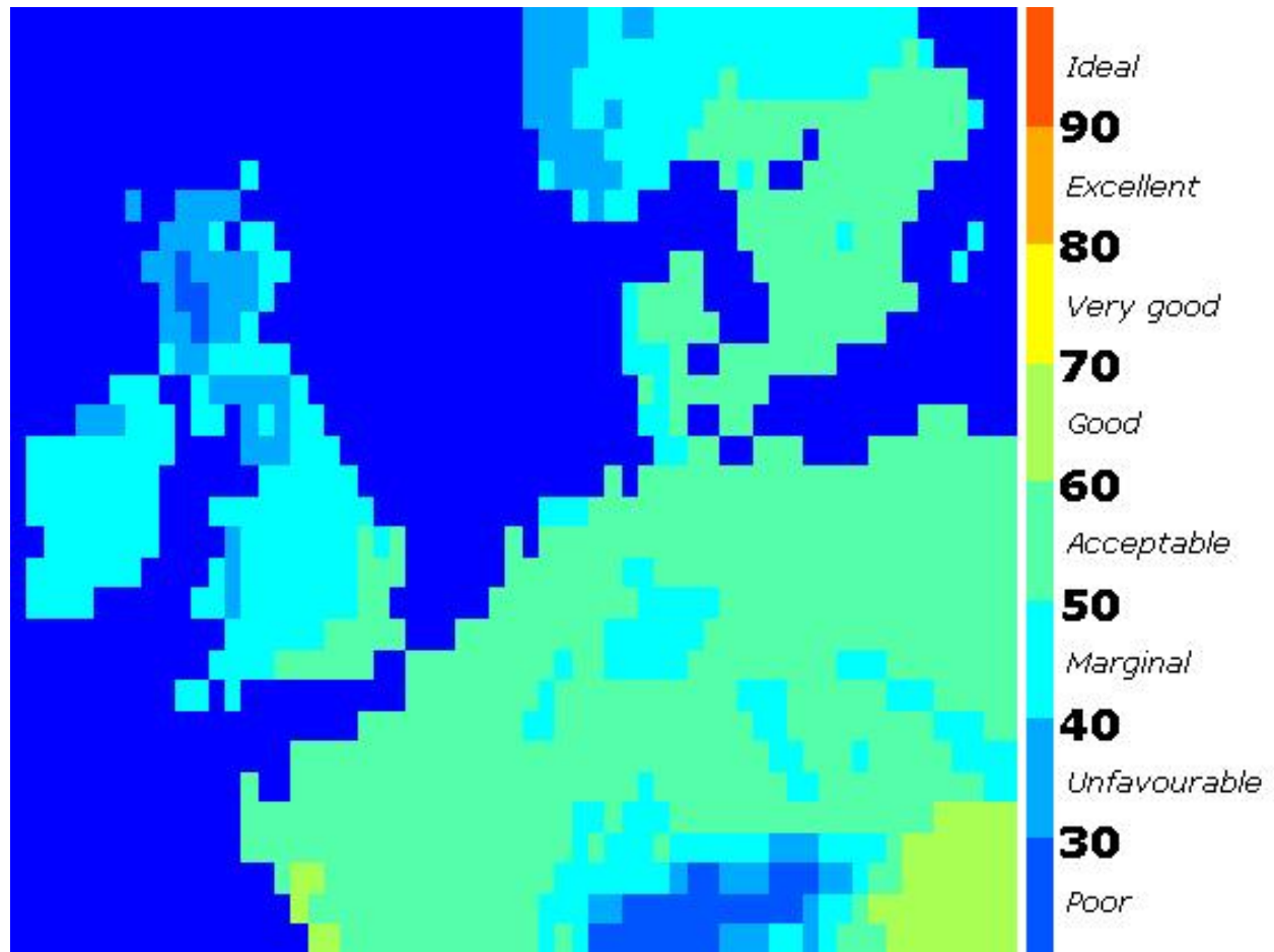
Figure 16. TCI Values for North-Western Europe (spring, 2080s, B1)
