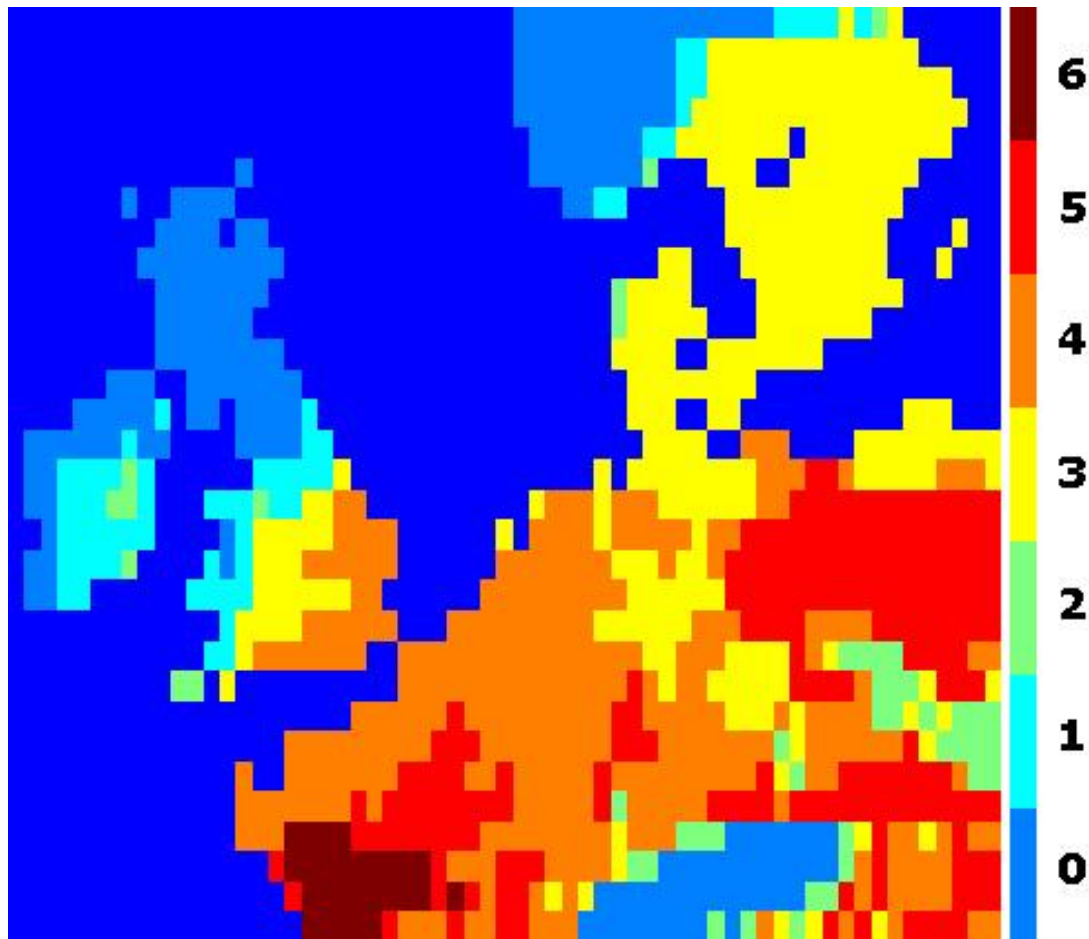
Figure 25. Number of Acceptable Months ( TCI \geq 70 ) in North-Western Europe (2050s, B1)
