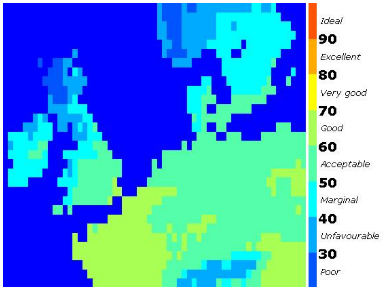
Figure 15. TCI Values for North-Western Europe (autumn, 2050s, A1F)
