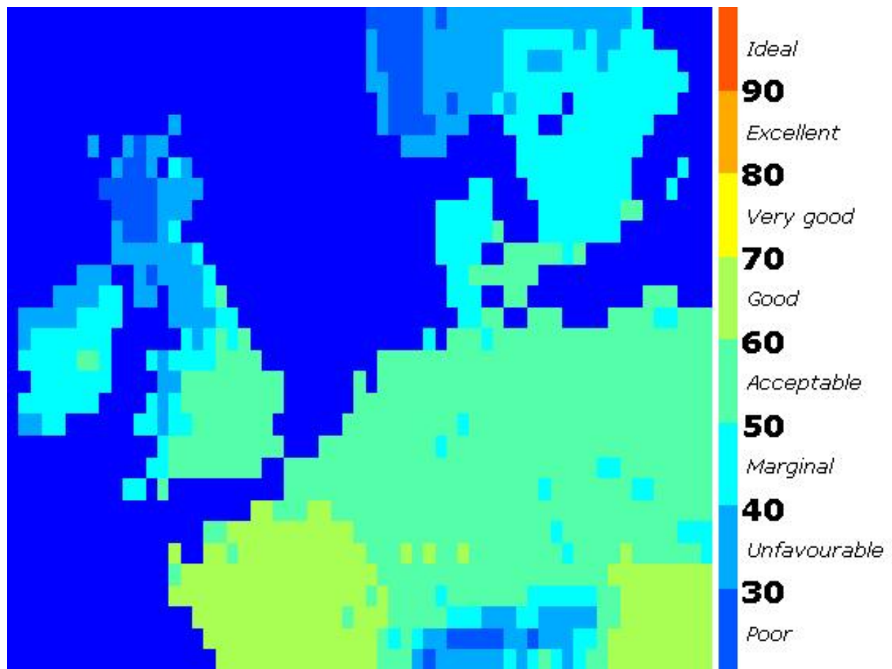
Figure 18. TCI Values for North-Western Europe (autumn, 2080s, B1)
