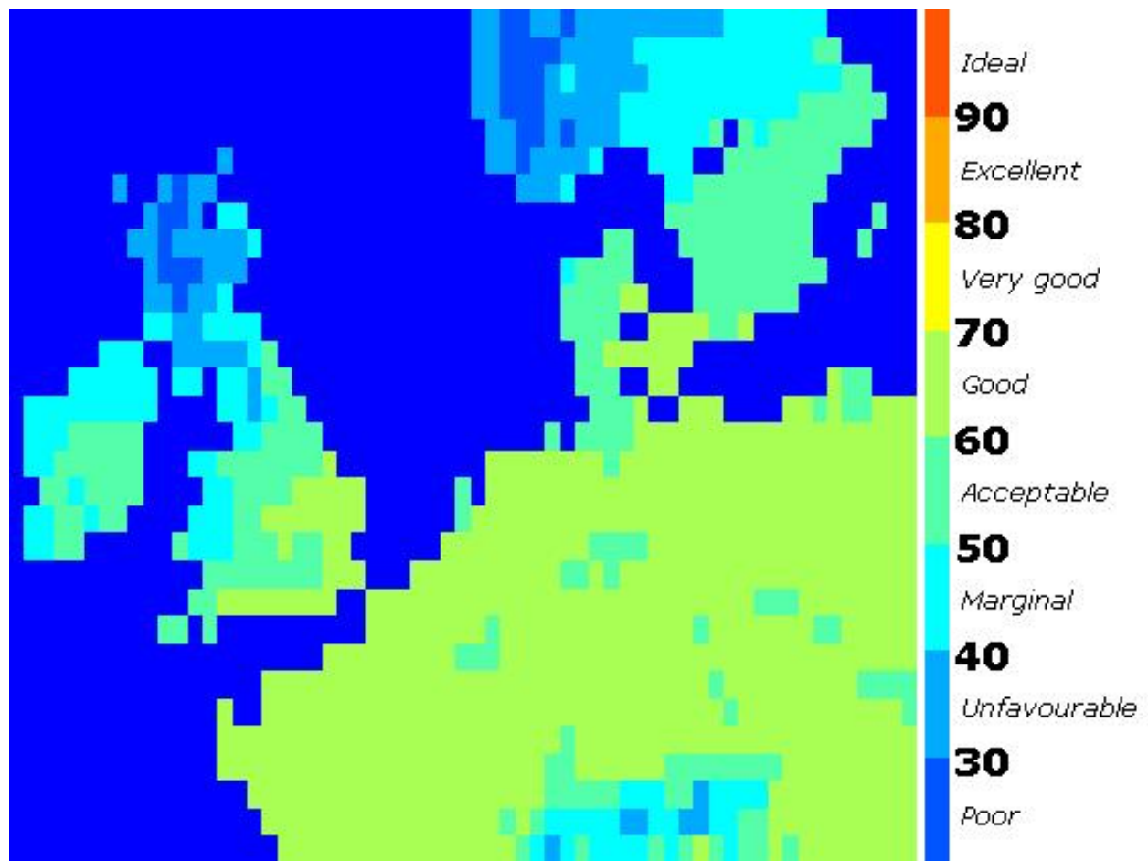
Figure 21. TCI Values for North-Western Europe (autumn, 2080s, A1F)
