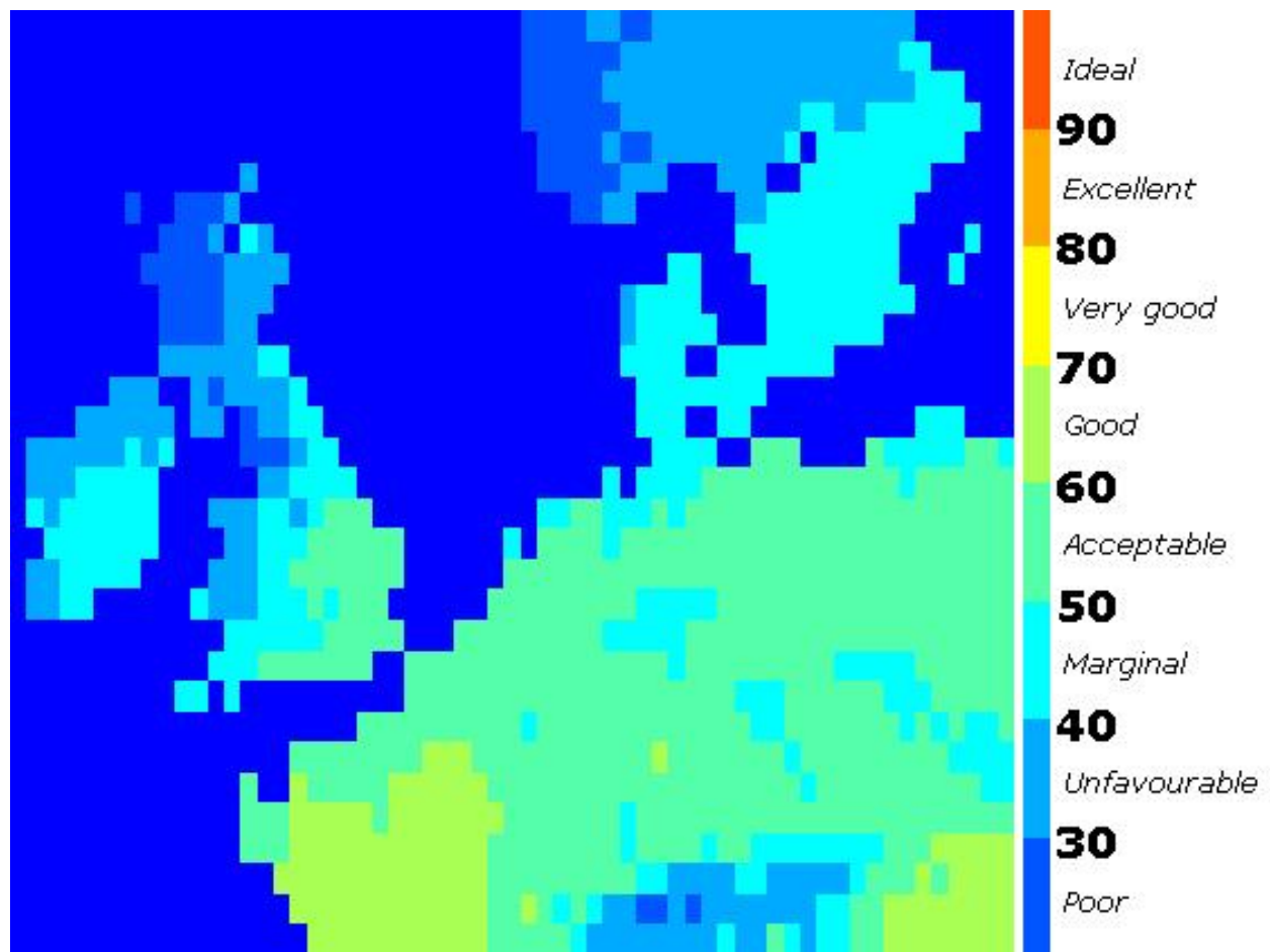
Figure 12. TCI Values for North-Western Europe (autumn, 2050s, B1)
