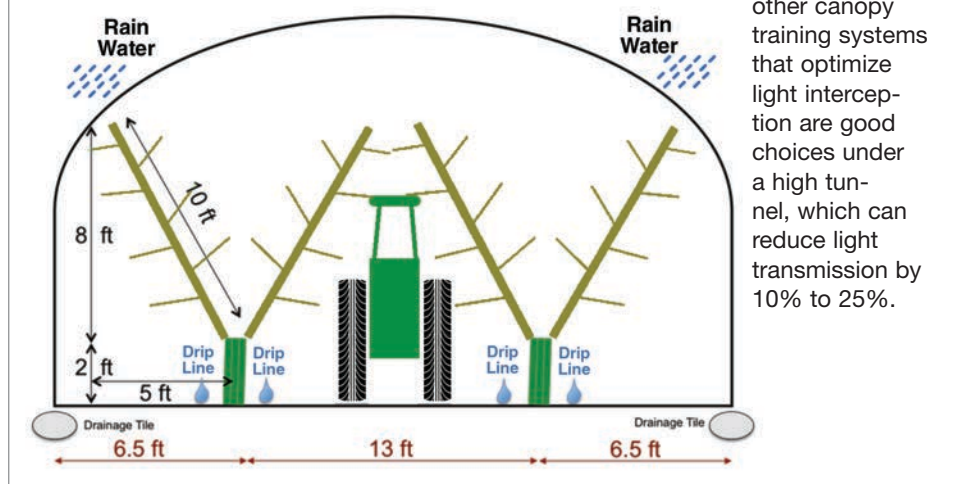
Figure 2 Training Canopies For High Tunnels
