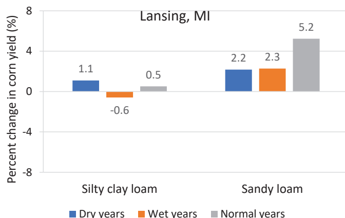
Figure 6- Percent change in 30-year average corn yield (2.5-ft shallow drains minus 4.1-ft deep drains). Shallow drains can increase corn yield in dry years and reduce yield in wet years. Shallow drains reduce year-to-year yield variability.
