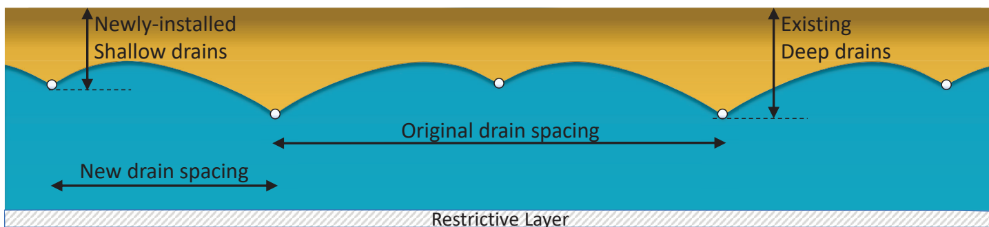
Figure 8- A bi-level drainage system where the original deep drains work in combination with the new shallow drains.
