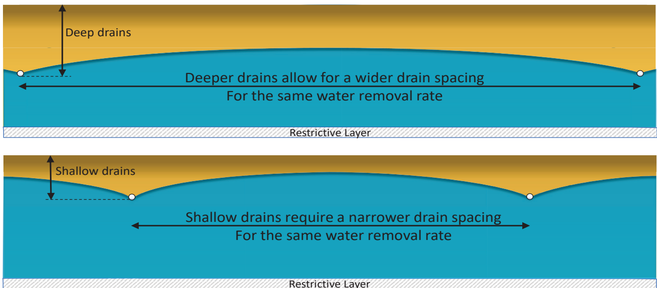
Figure 1- Shallow drains require a narrower drain spacing to achieve the same water removal rate as in a system with wider-spaced, deeper drains.
