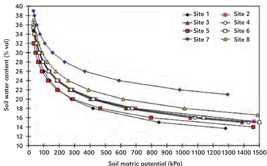
Figure 1. An example of soil-water retention curve developed to convert soil matric potential to soil water content for various soil textures.
