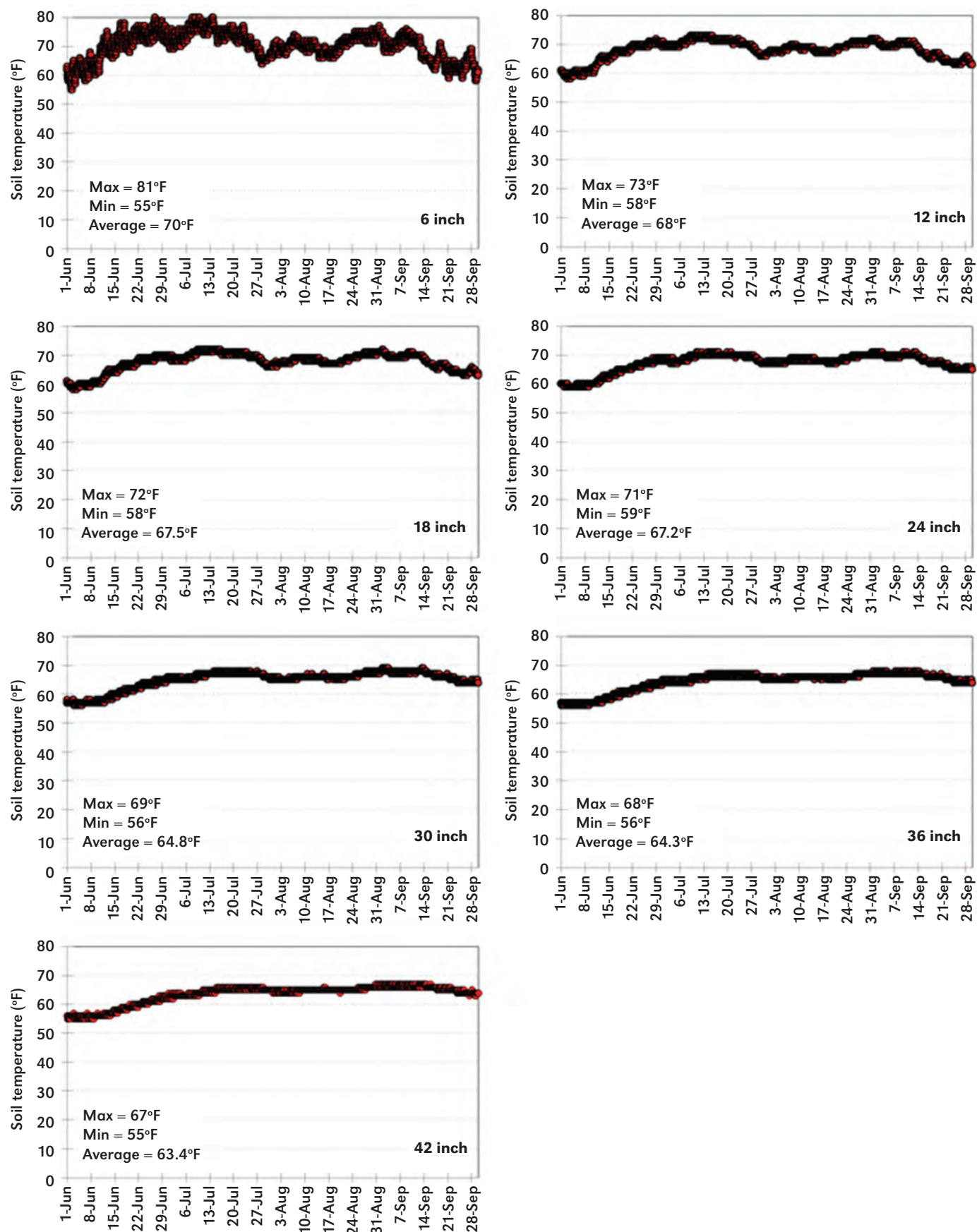
Figure 7. Soil temperature measured on an hourly basis at 6, 12, 18, 24, 30, 36, and 42 in soil layers on Hastings silt loam soil at the South Central Agricultural Laboratory, Clay Center, Neb.
