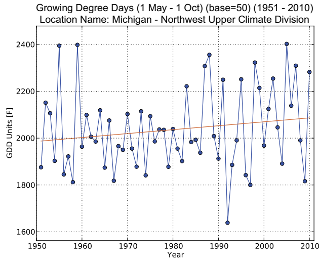
Figure 4 - Number of growing degree days from May 1 to October 1 across Northwest Upper Michigan from 1951 to 2010
