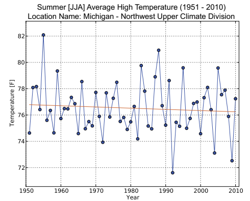
Figure 6. Region-wide temperature trends across Northwest Upper Michigan from 1951 to 2010 for summer daily maximum temperature (right), summer daily minimum temperature (below left), winter daily maximum temperature (below center), and winter daily minimum temperature (below right)
