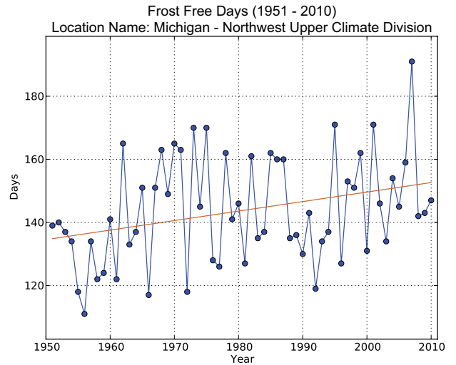
Figure 3 - Number of frost-free days across Northwest Upper Michigan from 1951 to 2010
