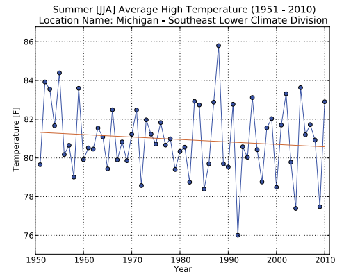
Figure 6. Region-wide temperature trends across Southeast Lower Michigan from 1951 to 2010 for summer daily maximum temperature (right), summer daily minimum temperature (below left), winter daily maximum temperature (below center), and winter daily minimum temperature (below right)
