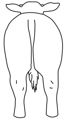
Figure 4: heavy-boned animal
