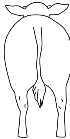
Figure 3: frail-boned animal
